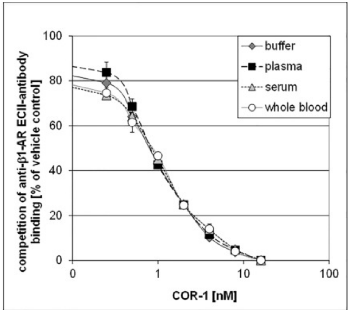
Fig 3. ELISA: Inhibition of anti- \beta_1 -AR EC2-antibody binding to coated 25-meric \beta_1 -AR peptides in the presence of increasing concentrations of COR-1, on a background of either 25% saline or rat serum, rat plasma or rat whole blood.
